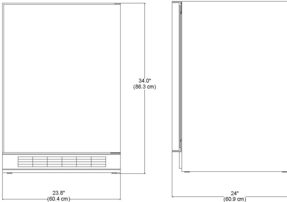
6.1 cu. ft. Refrigerator Reference Drawings
