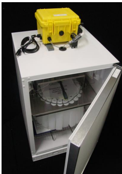
YB Multi-bottle Sampler on 6.1 cu. ft. White
